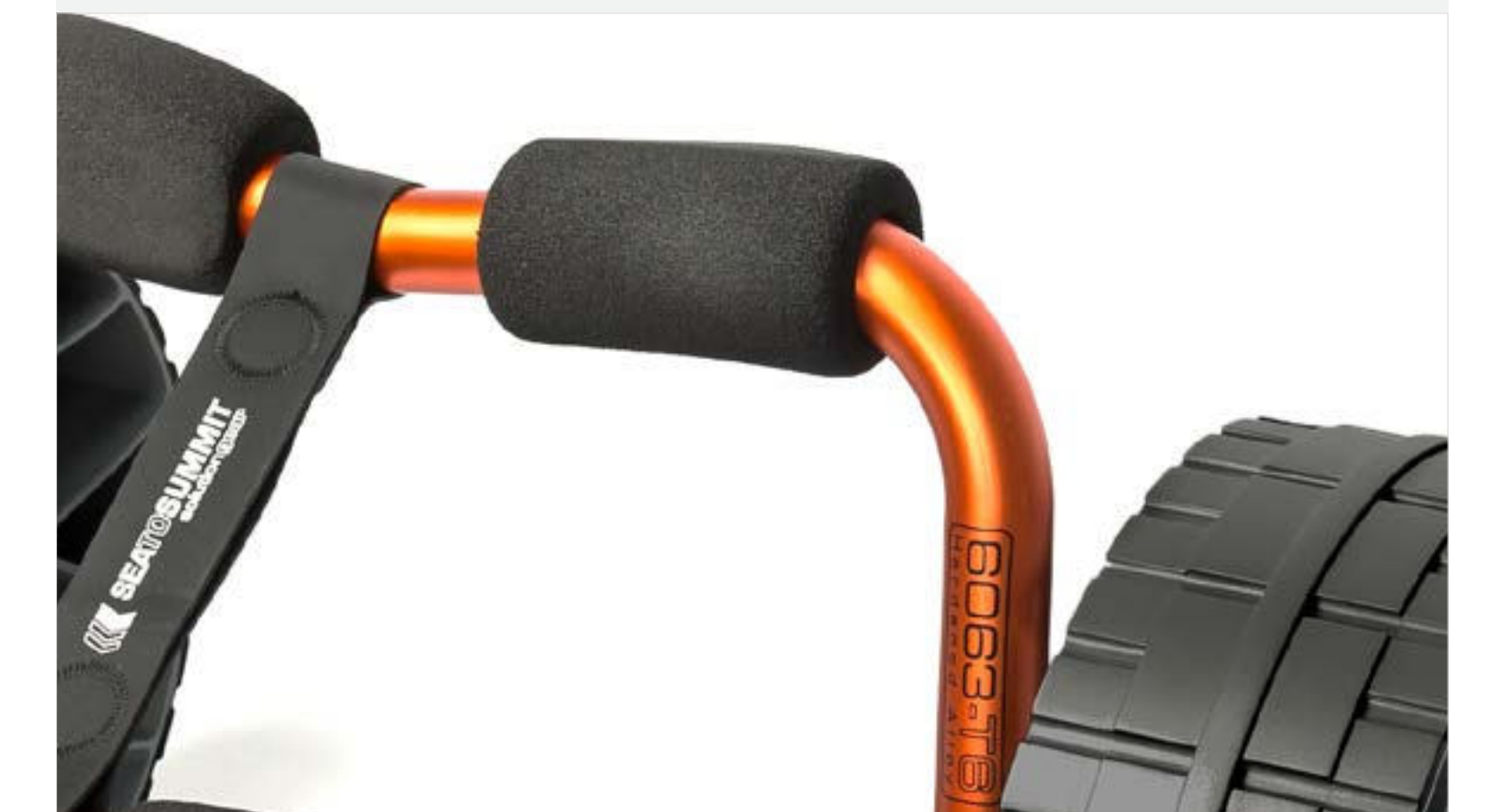
Oversized anodised 6063-t6 alloy tubing
